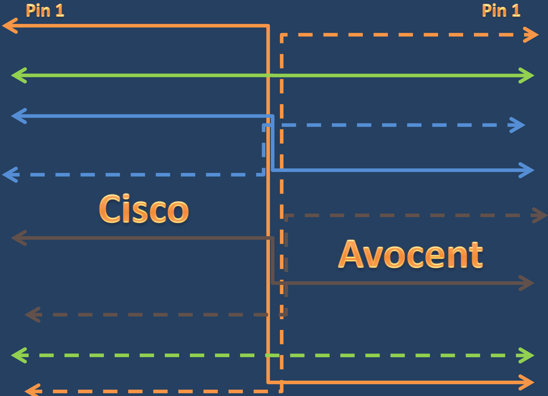
Avocent CCM 1650 to Cisco console ( rj-45/rj-45 patchcord pinout)
